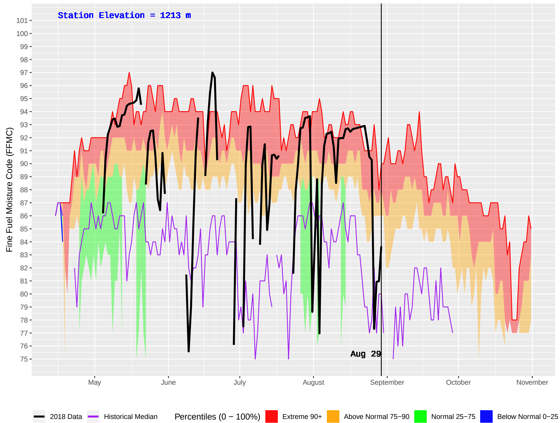
INGENIKA POINT (145) : Historical (1971–2016) and Current (2018) Daily Fine Fuel Moisture Code (FFMC)
