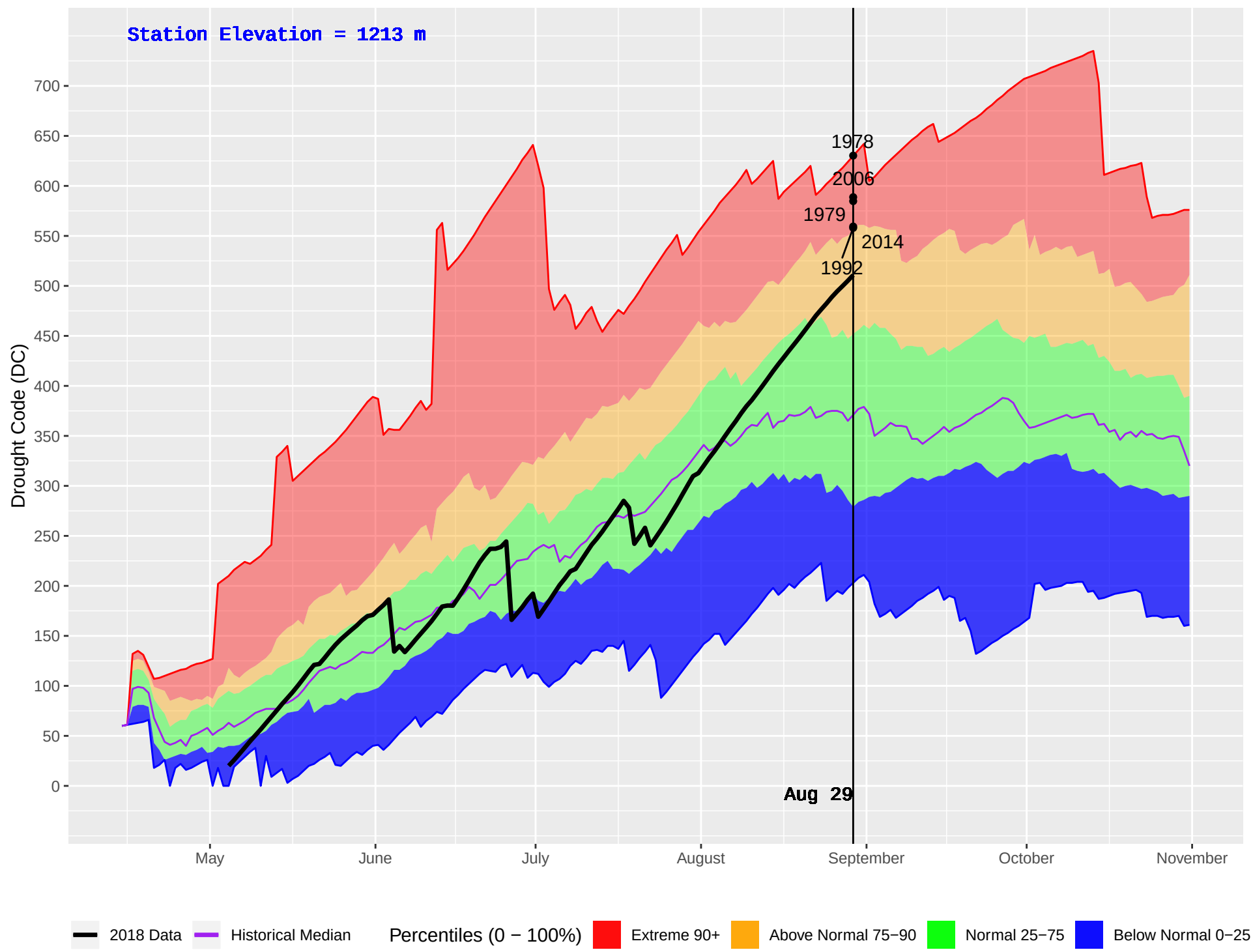
INGENIKA POINT (145) : Historical (1971–2016) and Current (2018) Daily Drought Code (DC)
